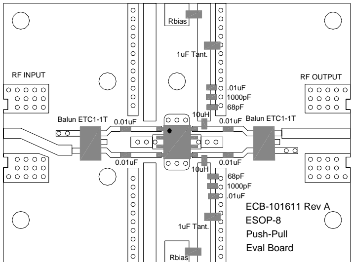
5-100 MHz Evaluation Board Layout
